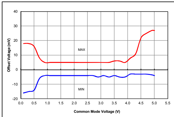
FIGURE 38-55: Comparator Offset, NP Mode ( CxSP = 1 ), V_{DD} = 5.5V , Typical Measured Values from -40^\circ C to 125^\circ C , PIC16F18856/76 Only.
