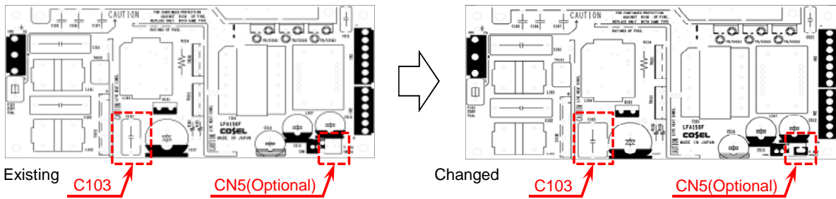
Fig.2.2 Silkscreen (PCB)
