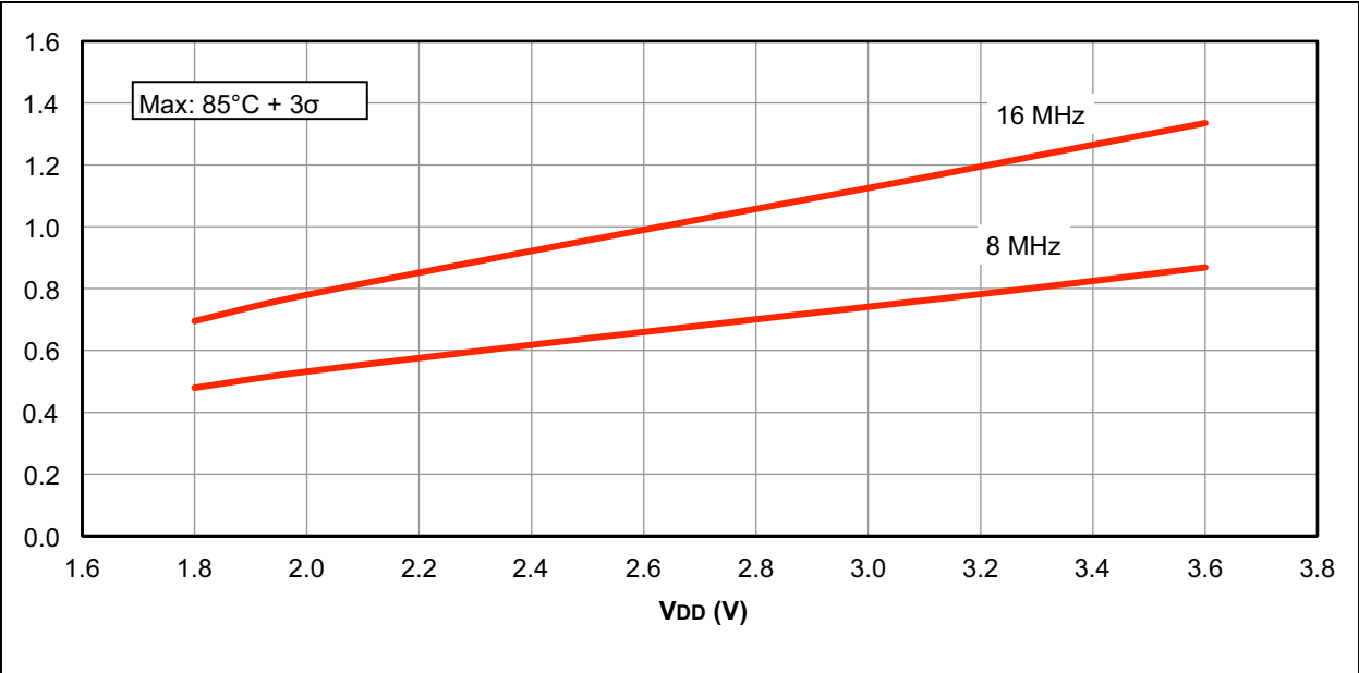
FIGURE 22-9: I DD , MAXIMUM, HFINTOSC
